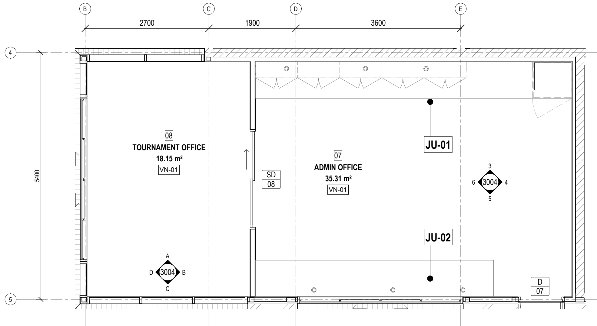
1 PLAN ROOM LAYOUT - ADMIN / TOURNAMENT OFFICE Scale: 1 : 50
