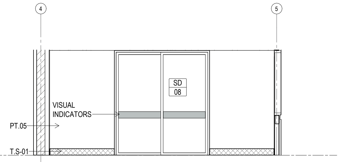
B ELEVATION TOURNAMENT OFFICE Scale: 1 : 50
