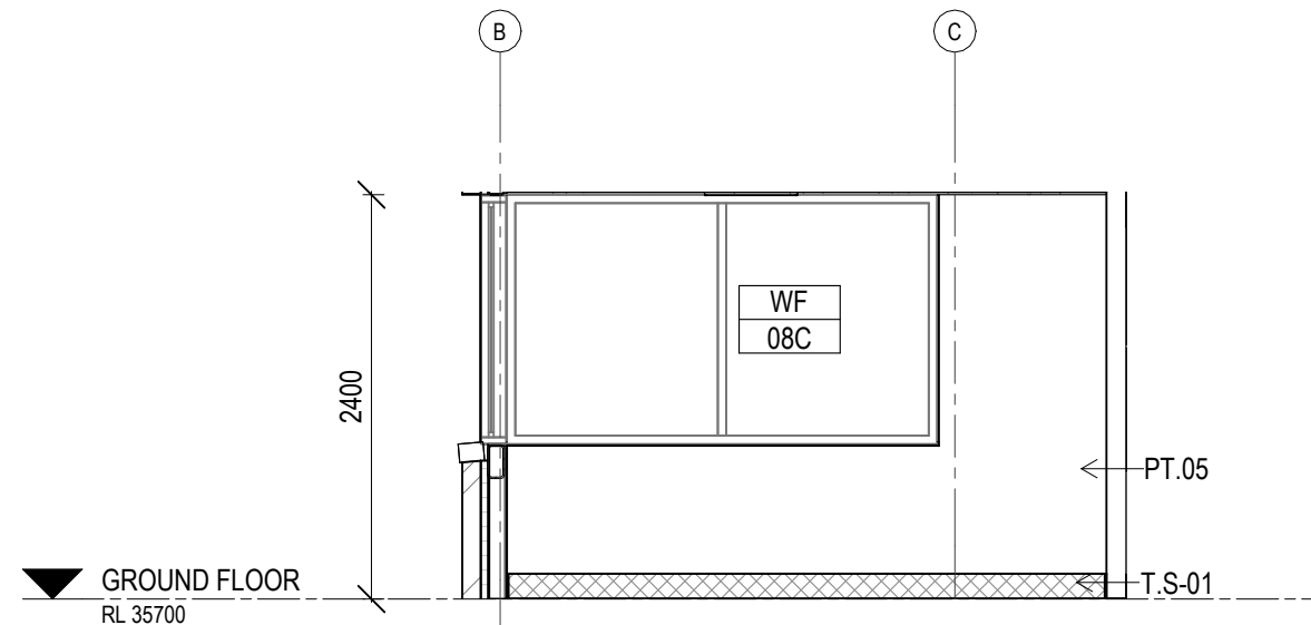
A ELEVATION TOURNAMENT OFFICE Scale: 1 : 50
