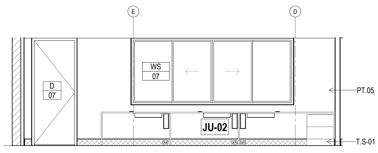
5 ELEVATION ADMIN OFFICE Scale: 1 : 50
