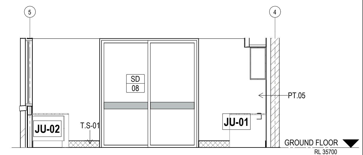
6 ELEVATION ADMIN OFFICE Scale: 1 : 50
