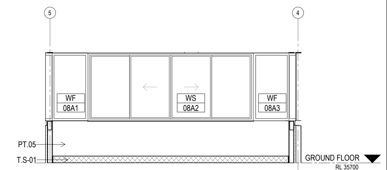
D ELEVATION TOURNAMENT OFFICE Scale: 1 : 50
