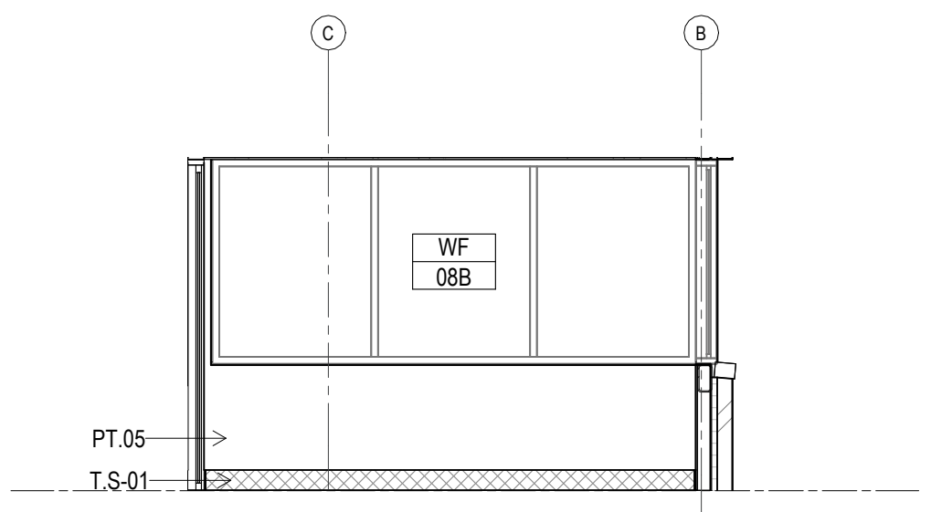
C ELEVATION TOURNAMENT OFFICE Scale: 1 : 50
