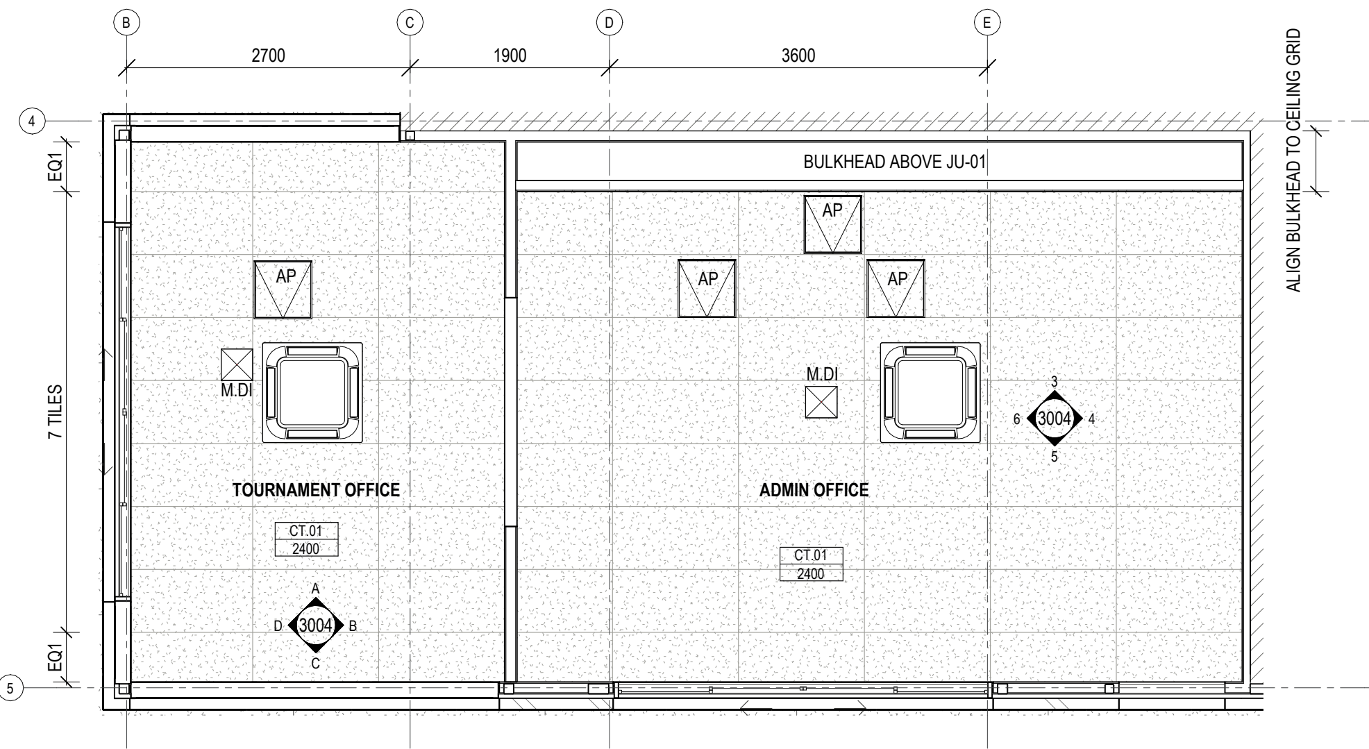
2 REFLECTED CEILING PLAN ROOM LAYOUT - ADMIN / TOURNAMENT OFFICE Scale: 1 : 50
