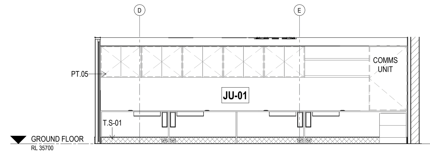
3 ELEVATION ADMIN OFFICE Scale: 1 : 50
