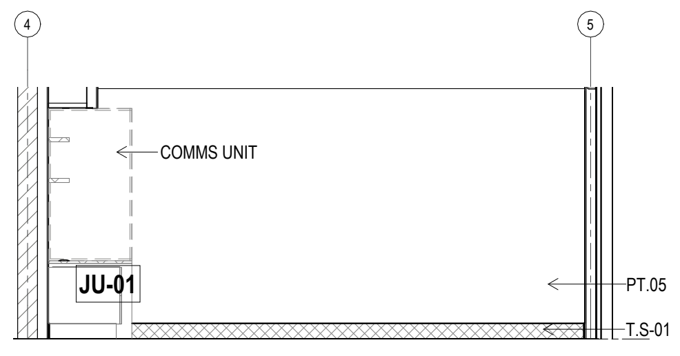
4 ELEVATION ADMIN OFFICE Scale: 1 : 50
